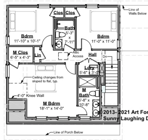
Living Area this Floor: 857 sq ft 8 ft Ceilings
