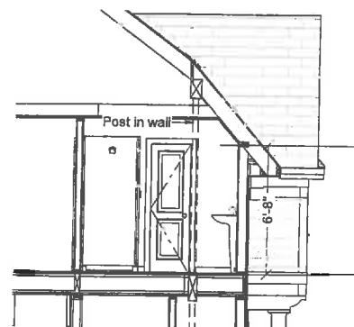
Section @ Small Bath
