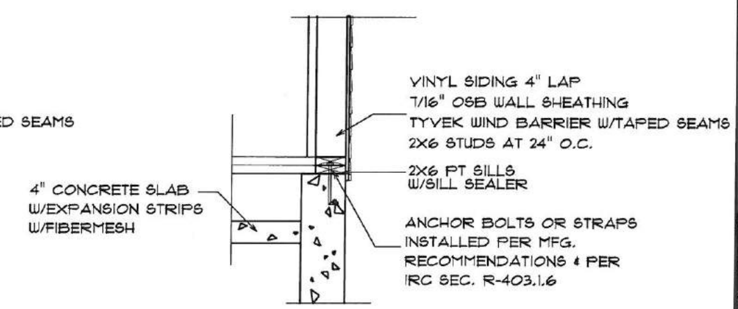
DETAIL "G"
