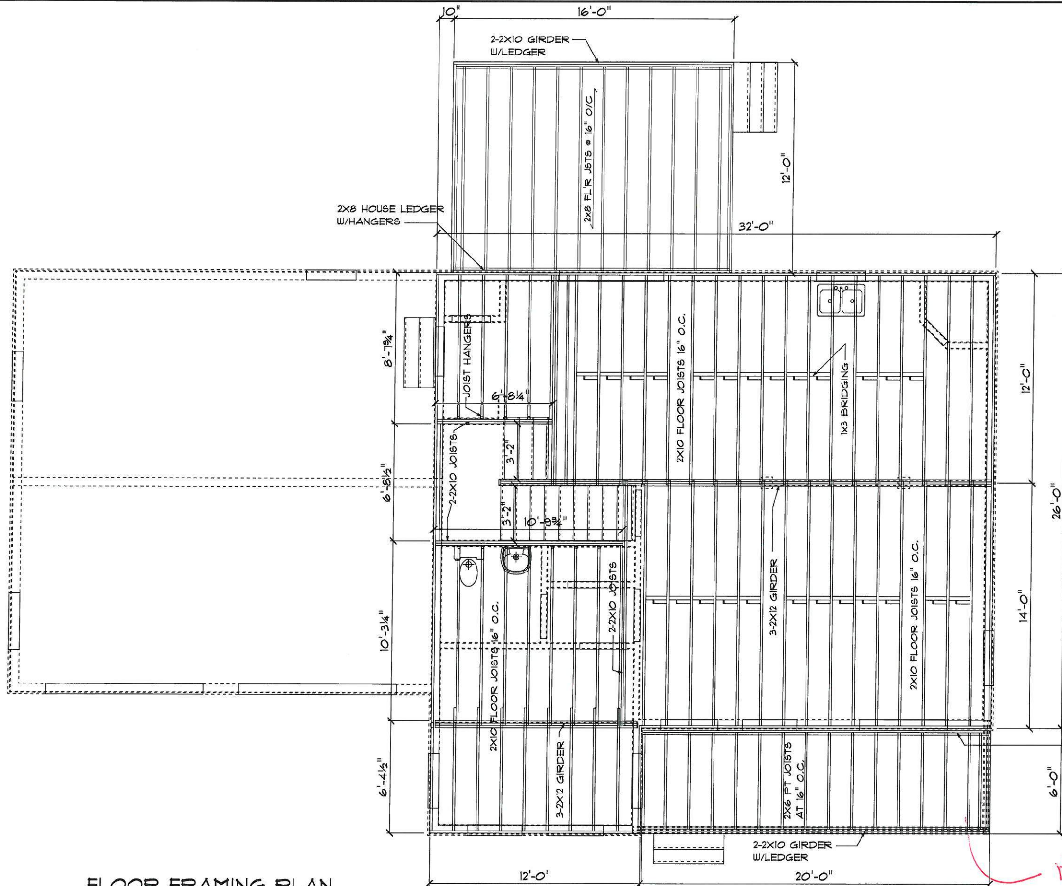
FLOOR FRAMING PLAN SCALE: 3/16" = 1'-0"
