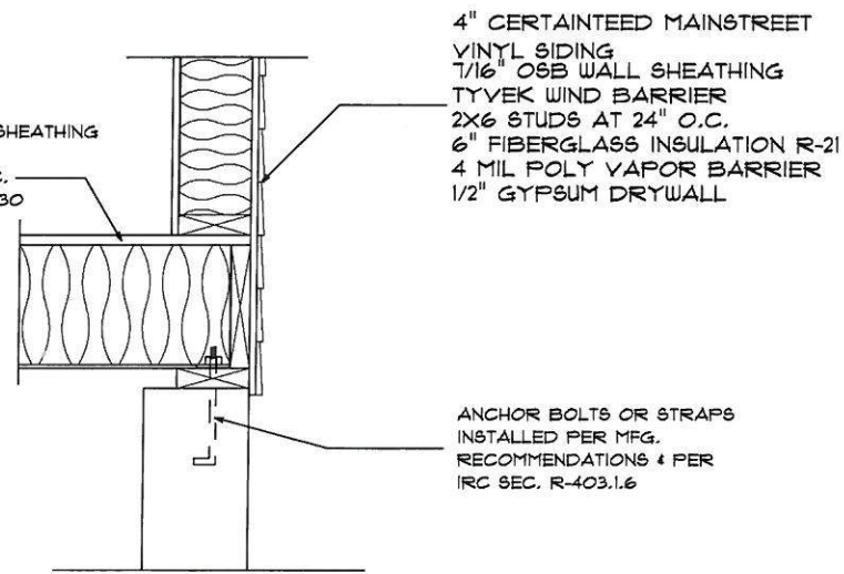
DETAIL "C" SCALE: 3/16" = 1'-0"
