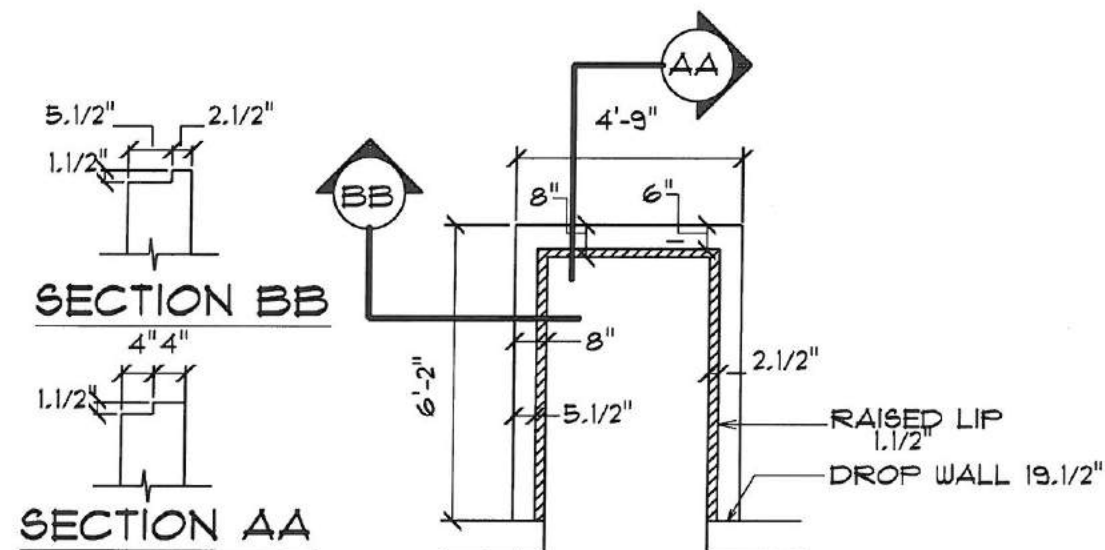
BULKHEAD DETAIL
