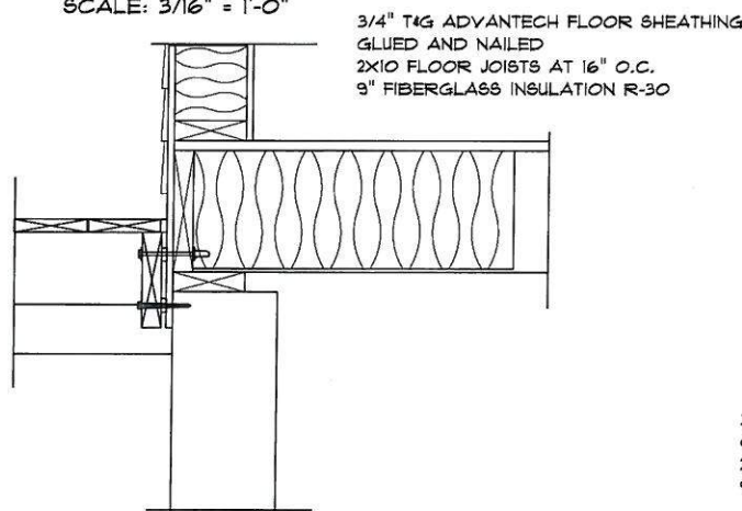
DETAIL "B" SCALE: 3/16" = 1'-0"
