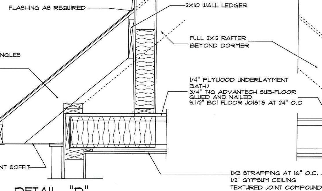
DETAIL "D" SCALE: 3/16" = 1'-0"
