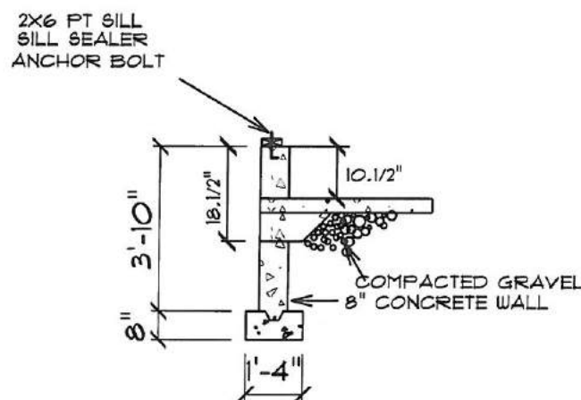
DETAIL "D"
