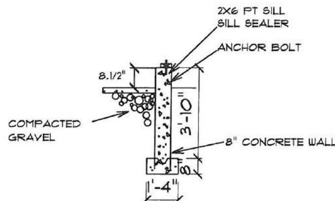
DETAIL "C"
