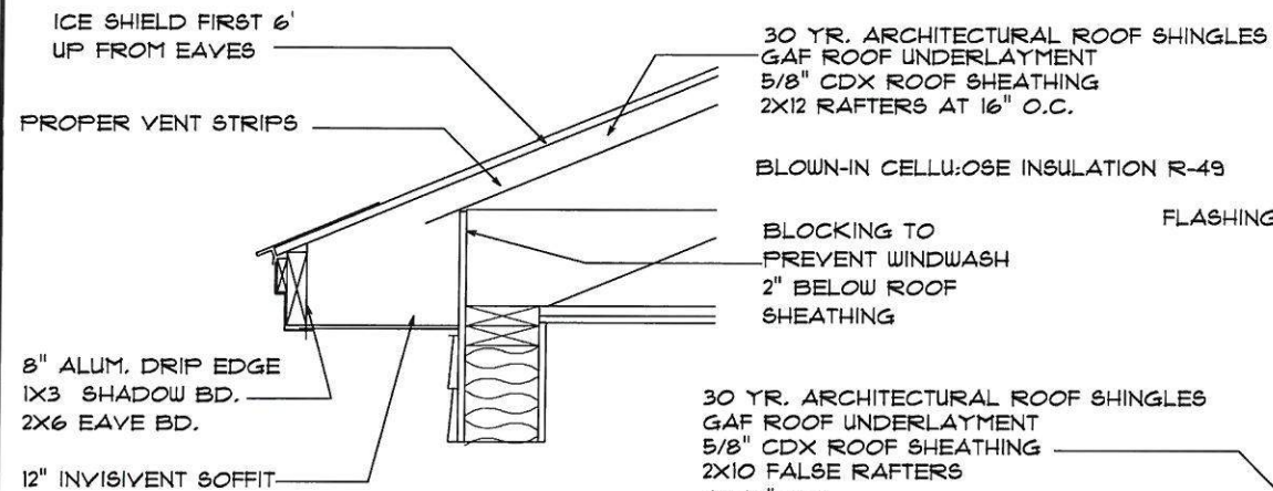
DETAIL "F" SCALE: 3/16" = 1'-0"
