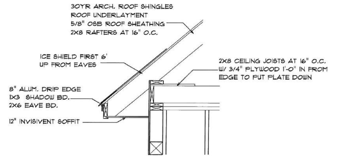
DETAIL "H"
