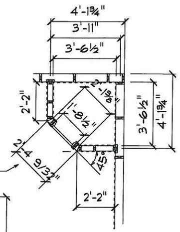
PANTRY WALL DETAIL SCALE: 3/16" = 1'-0"
