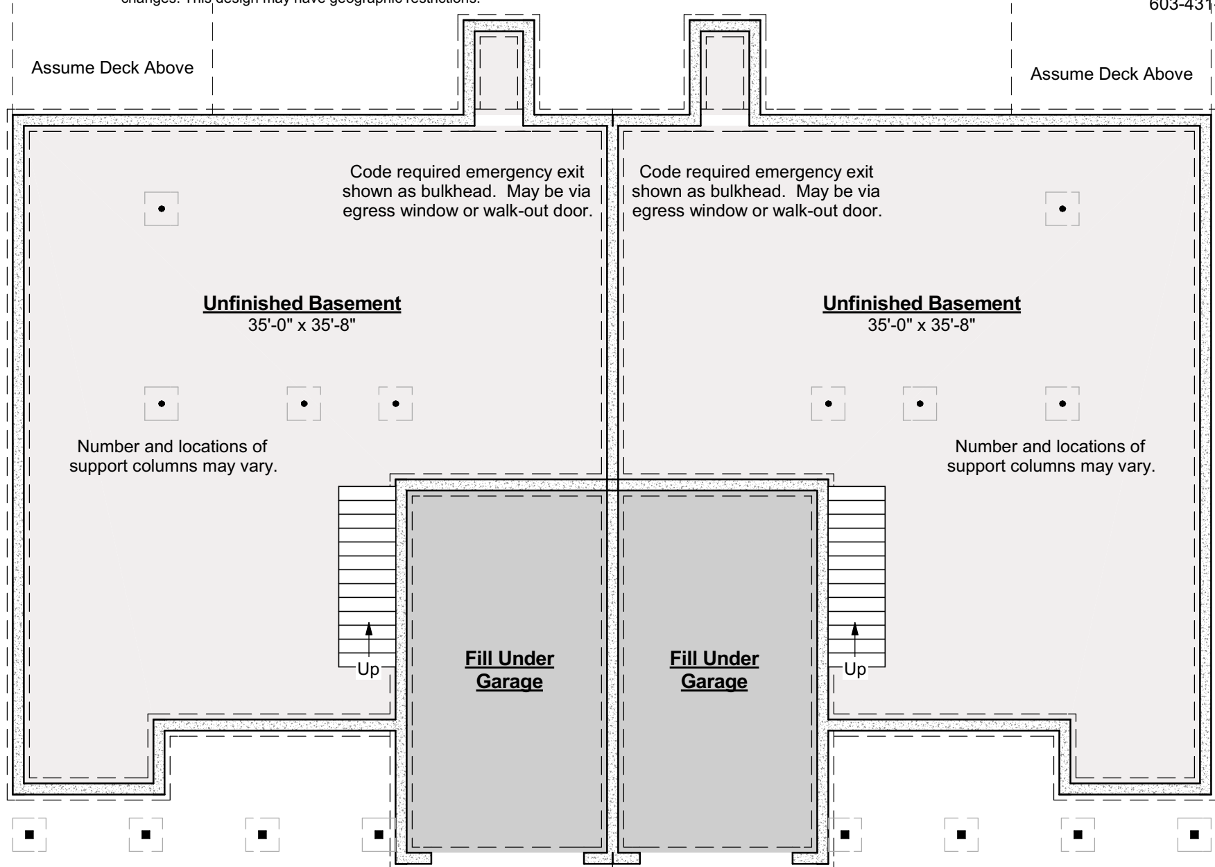
Foundation Plan
