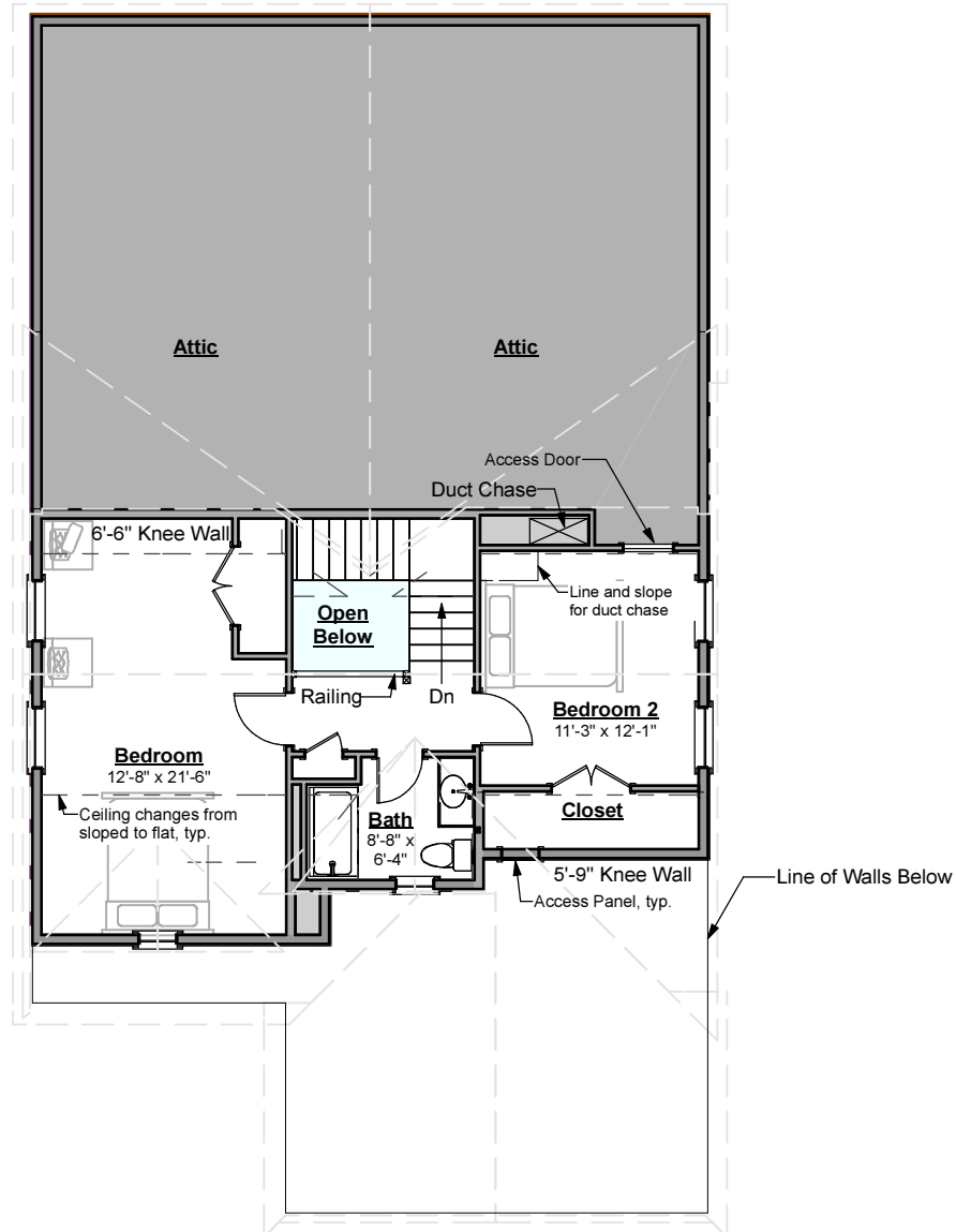
Living Area - Second Floor: 708 SF
